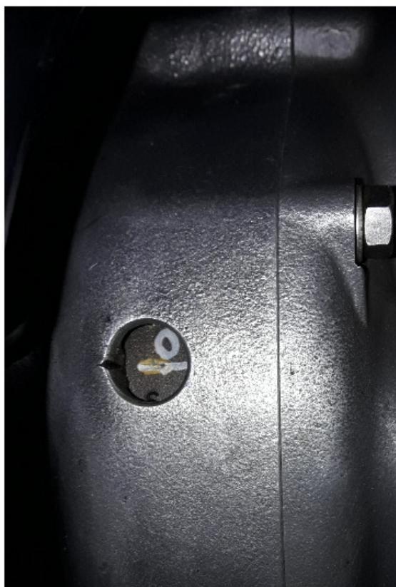
Picture 4 – Setting the Advance of ignition spark by setting the Trigger tooth position
