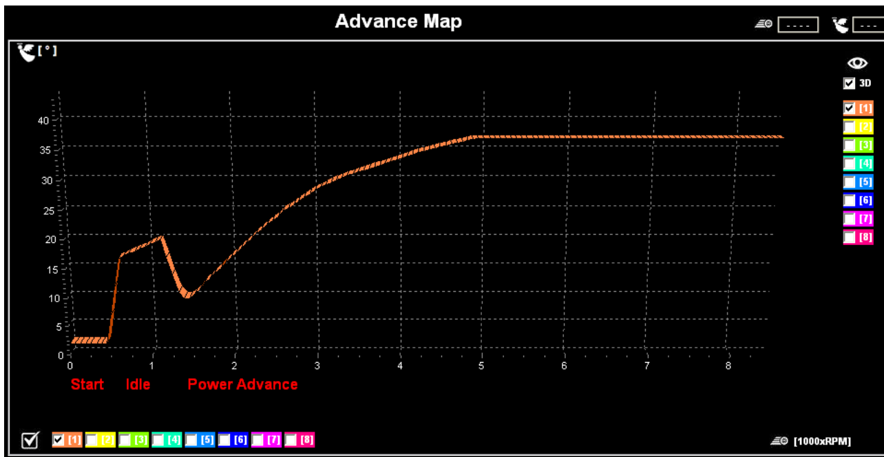
Picture 7 – ECU MASTER LITE – default advance curve
