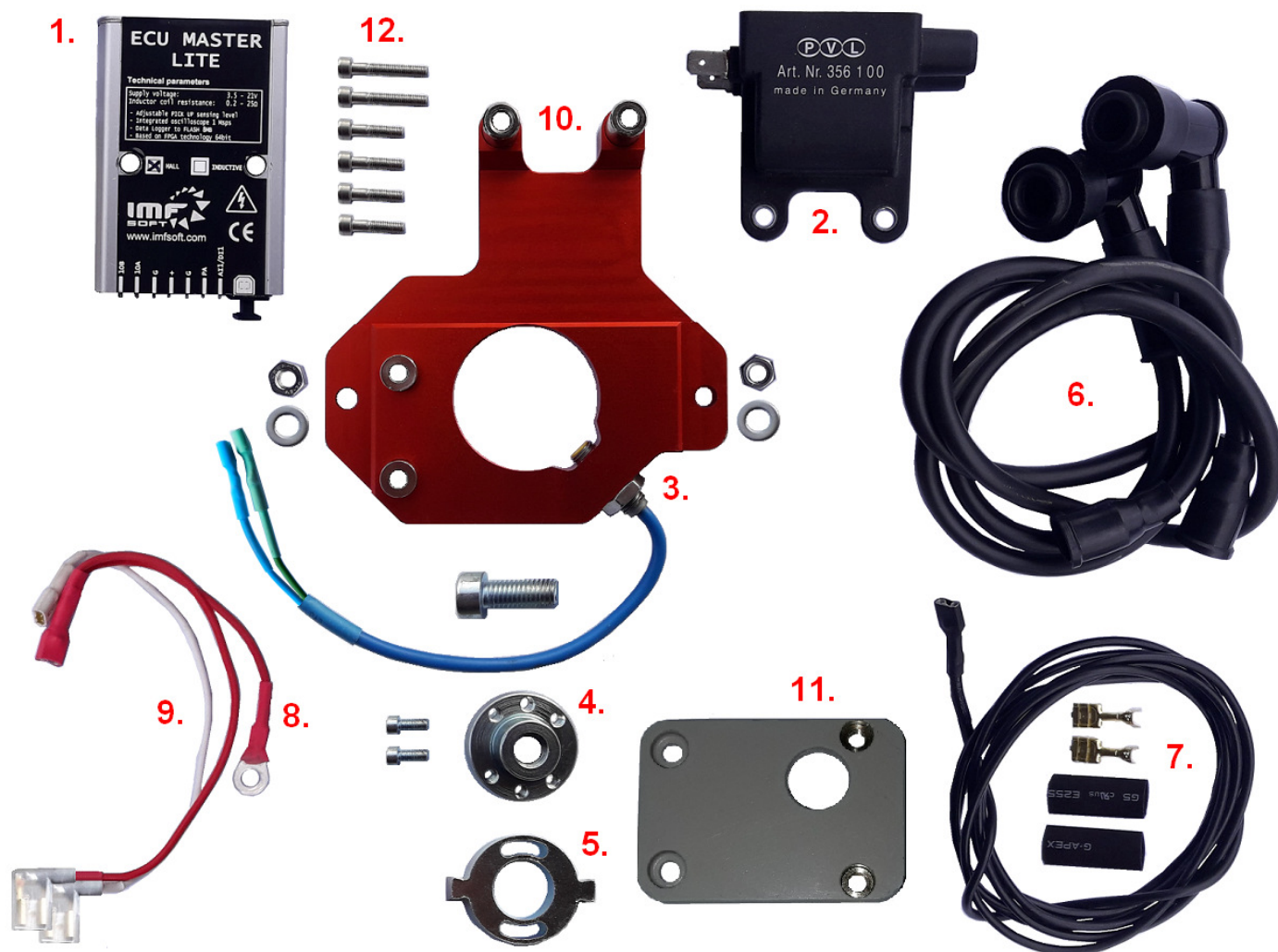
Picture 1 – Ignition Kit Parts
